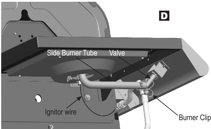
Correctly assembled burner-to-valve engagement
