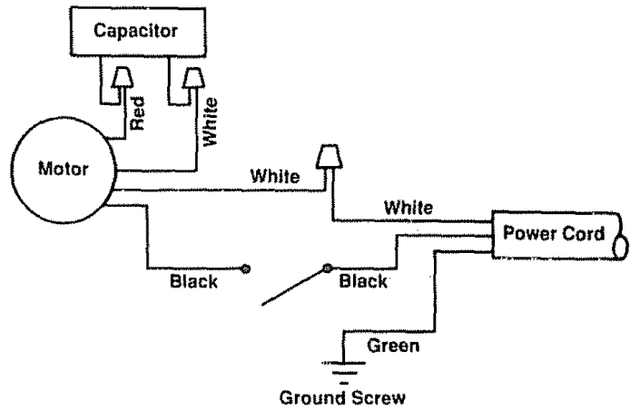
Wiring Diagram
