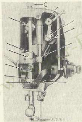
Fig. 25. End View, Showing Oiling Points 30
