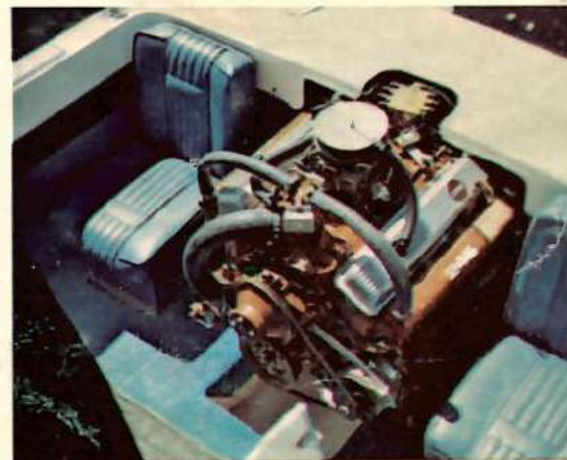
Engine installation in the FALCON 184 I/O showing access to engine and jump seats. Max HP shown.
